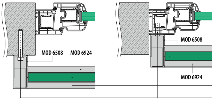
Facade mounting
