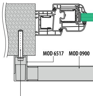
Facade mounting
