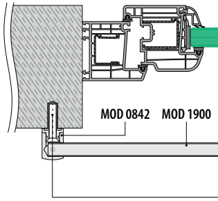
Facade mounting
