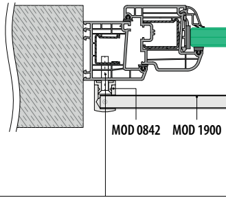
Frame mounting
